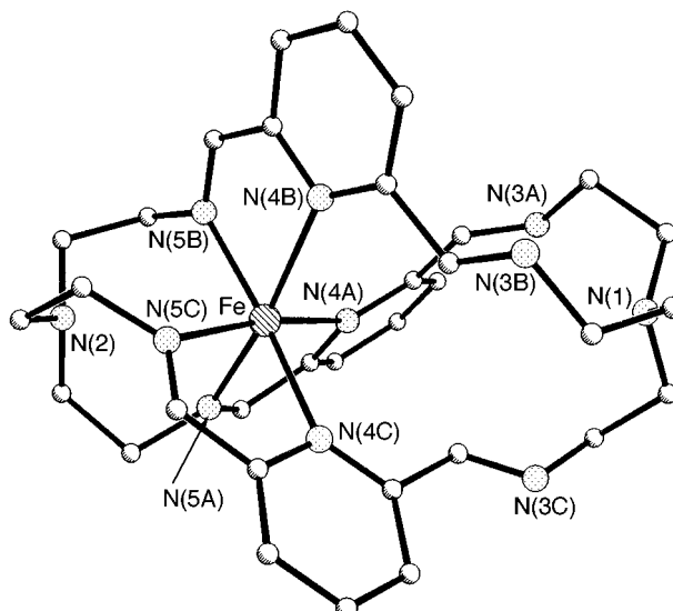
Fig. 1 Perspective view of the [FeL 1 ] 2+ cation. Hydrogen atoms are omitted for clarity
